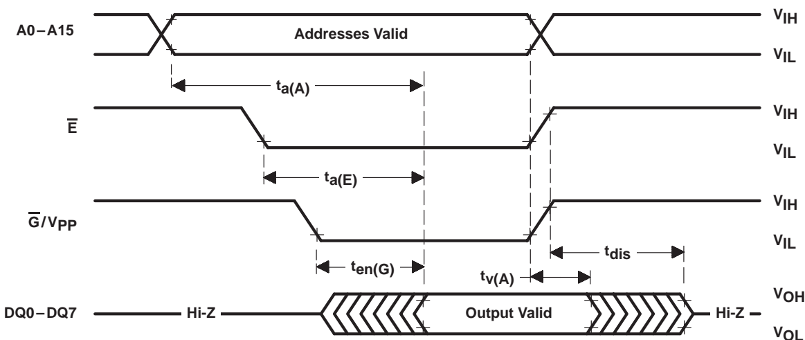
Figure 3. Read-Cycle Timing
