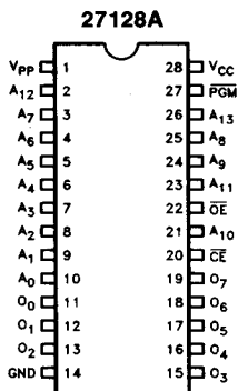
Figure 2. Cerdip(D) DIP Pin Configuration
