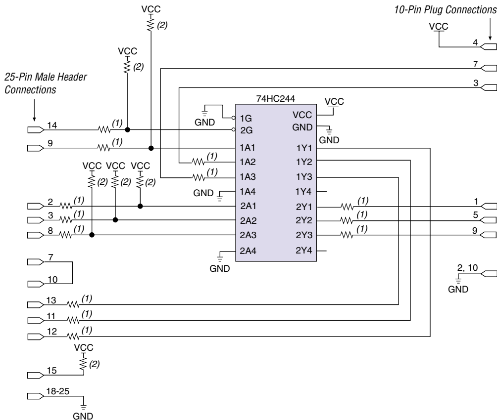
Figure 2. ByteBlasterMV Schematic
